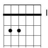
F minor
